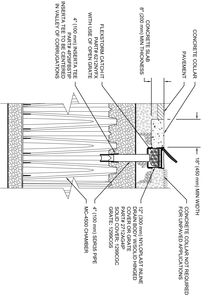
MC-4500 4" INSPECTION PORT DETAIL NTS
