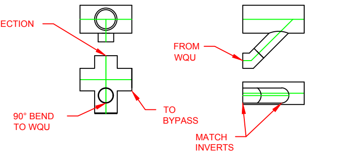
INLET STRUCTURE FABRICATED SUMP TEE
