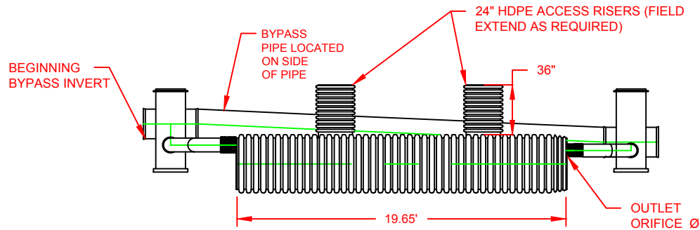
PROFILE VIEW
