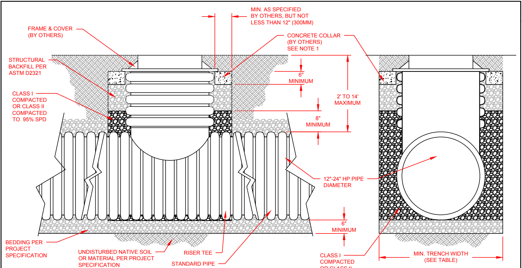
RECOMMENDED MINIMUM TRENCH WIDTHS
