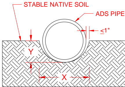
Figure 2 Rounded Trench Installation
