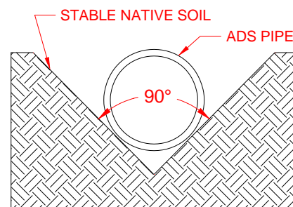
Figure 1 V-Bottom Trench
