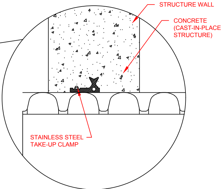
DETAILED CONNECTION VIEW
