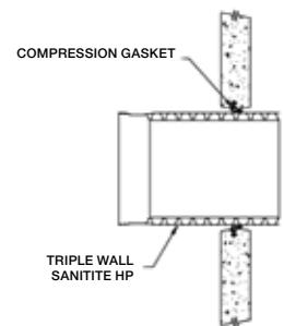
Compression Gasket Connection to Triple Wall Pipe
